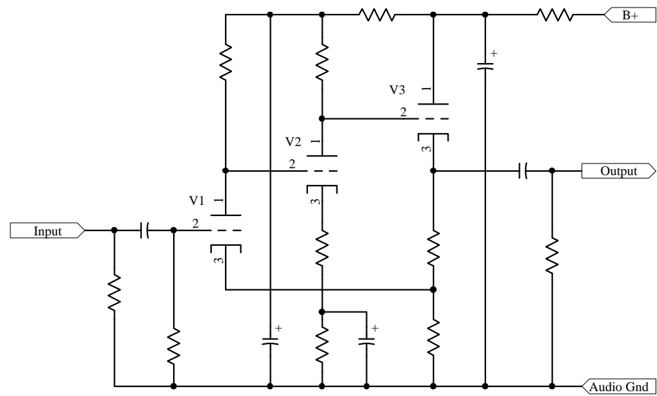
Vacuum tube example, from John Linsley Hood Figure 1
