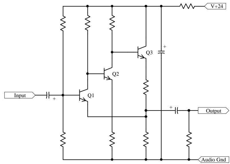
NPN middle stage variant Figure 2
