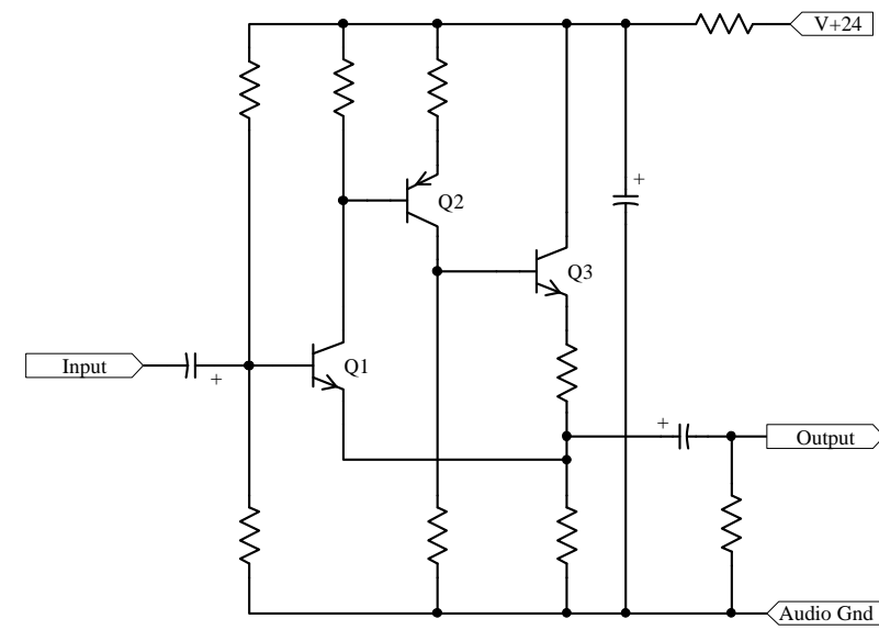
PNP middle stage variant Figure 3
