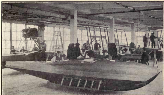
FIG. 14.—Building a flying boat hull. Note wing stumps and hydroplane fins.
